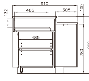
VMINPMR B caisse PMR
