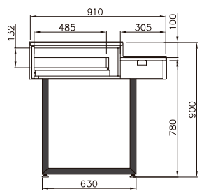
VMINPMR P caisse PMR
