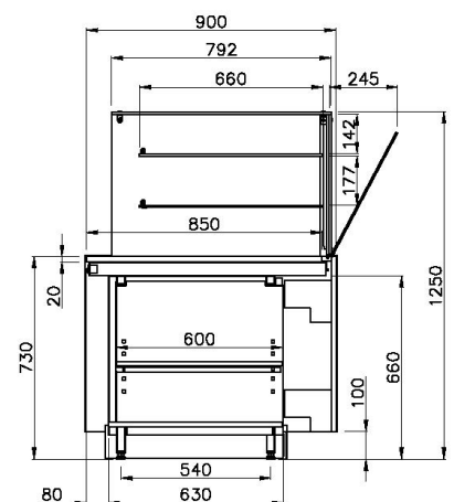
VMINPMR P caisse PMR
