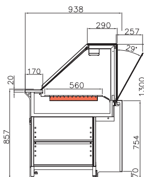
Vitrine chaude Version plaque chauffante
