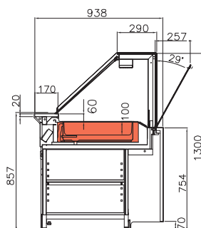
Vitrine chaude Version bain-marie
